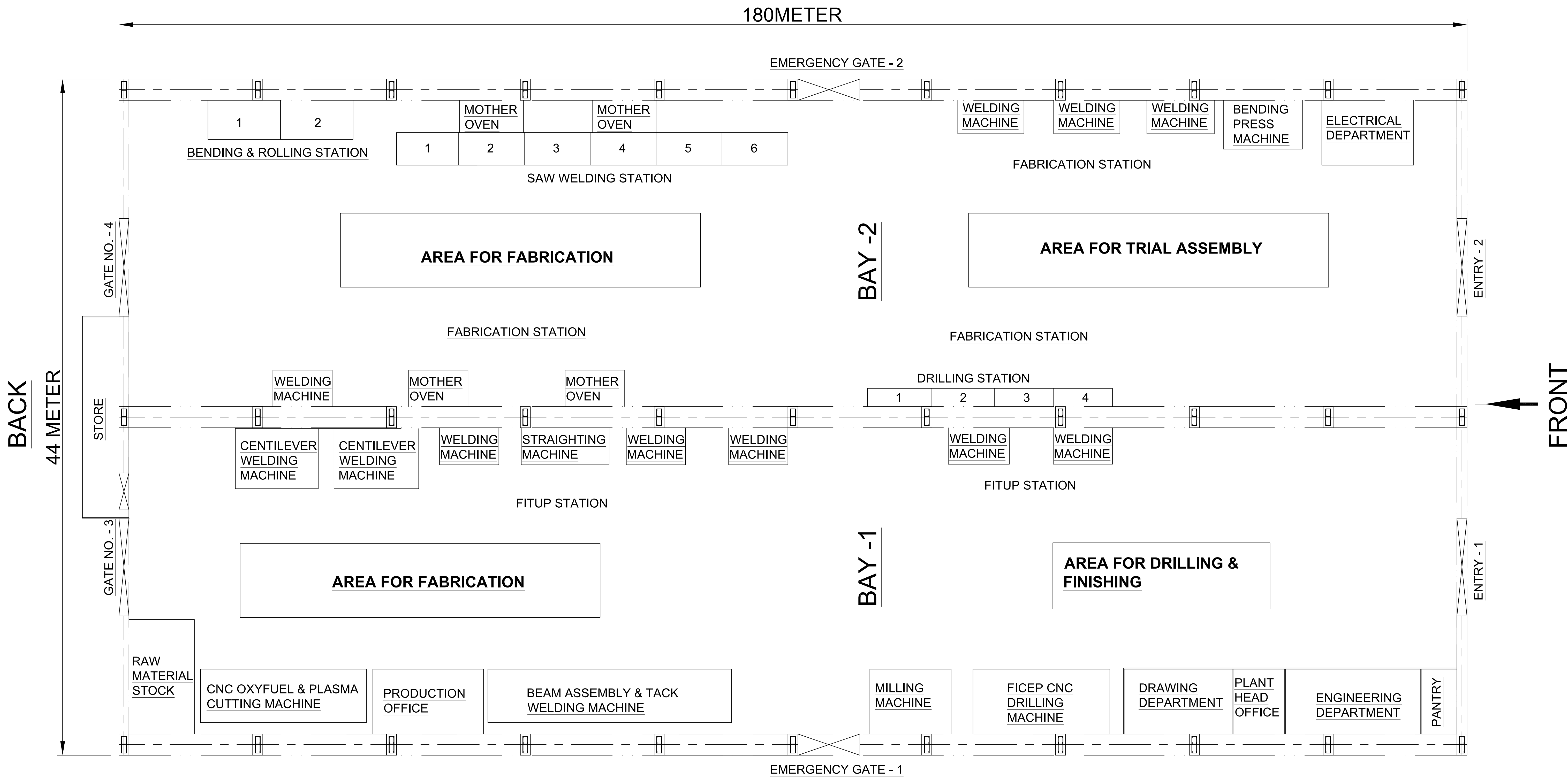
PLAN
